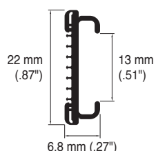
New Valance rail cross section with a Velcro (hooks)
