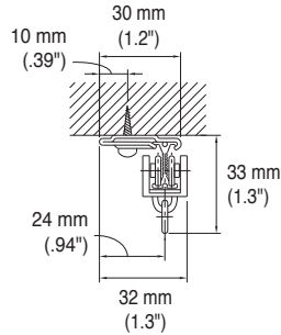
Ceiling Double Bracket Bracket width = 18 mm (.71")
