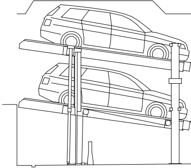
WÖHR Parklift 405-185 (315)
