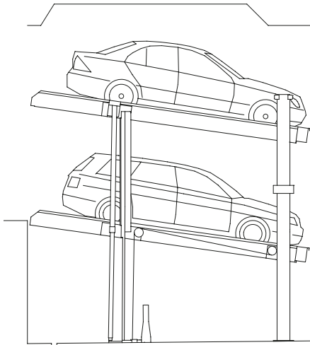
WOEHR Parklift 405-230 (405)
