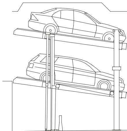
WOEHR Parklift 405-230 (360)
