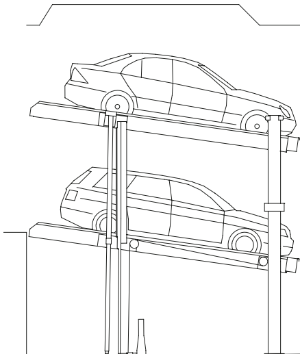
WOEHR Parklift 405-240 (440)
