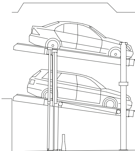
WOEHR Parklift 405-225 (410)
