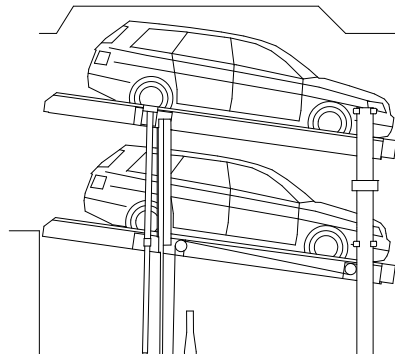
WÖHR Parklift 405-190 (330)
