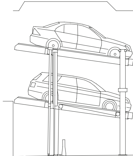
WOEHR Parklift 405-240 (435)
