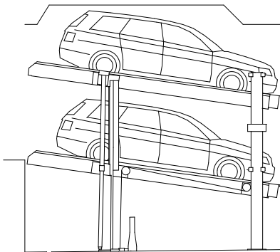
WÖHR Parklift 405-190 (320)
