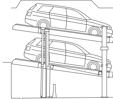
WÖHR Parklift 405-185 (320)
