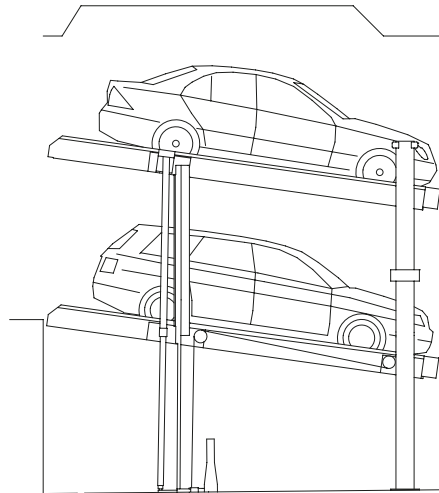
WOEHR Parklift 405-230 (415)
