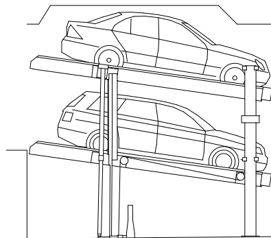
WÖHR Parklift 405-190 (310)
