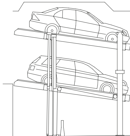
WOEHR Parklift 405-235 (365)
